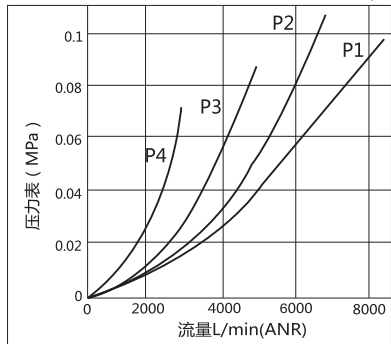
AF4000-06 3/4
