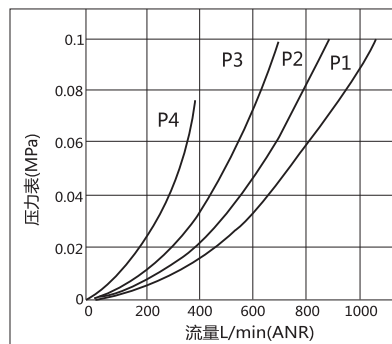
AF4000 3/8-1/2
